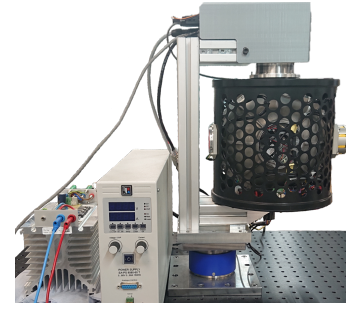
Fig. 5. Stationary experimental setup, where the SECMG is located on top of a multi-component sensor.
