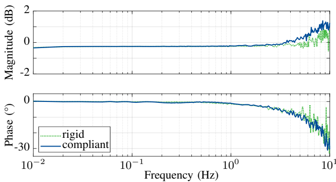
Fig. 7. Frequency response of the compliant and rigid CMG with respect to the multisine reference torque.
