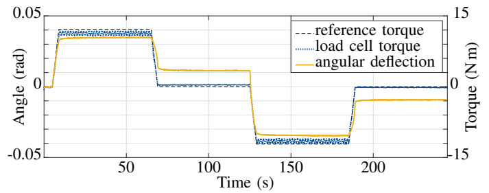
Fig. 8. Exemplary torque pulse experiment showing the torque tracking ability and the resulting angular deflection.
