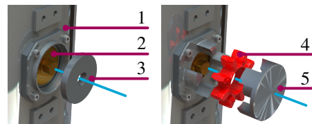
Fig. 3. Figure of the three options on the series coupling, where (1) is the gimbal frame and (2) the vacuum housing. Components (2) is rotationally contained via a P3G connection (acc. DIN 32711). Bottom left shows the locked option, where (3) is a solid disk. Bottom right is the viscoelastic option where (4) is the elastomer element and (5) the hub.
