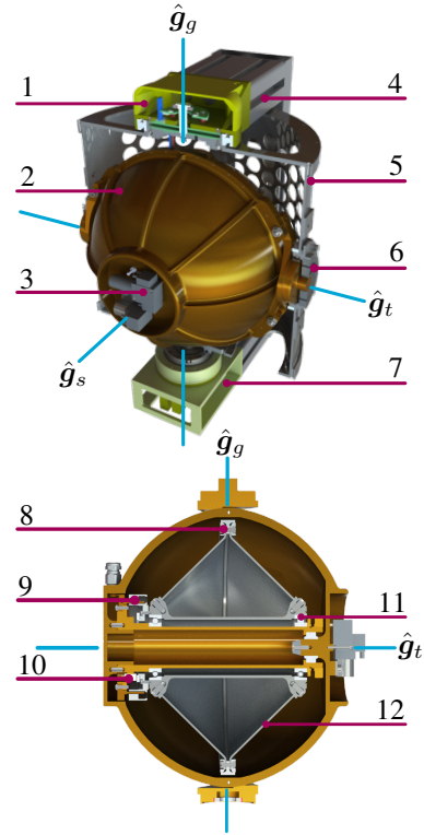
Fig. 2. The top figure shows a semi-cross-section of the whole device where (1) denotes the housing for the slip-ring and gimbal encoder, (2) the vacuum housing, (3) the vacuum-pump, (4) the device-frame, (5) the gimbal-frame, (6) the series coupling, and (7) the gimbal motor and gearbox. The bottom figure shows a cross-section of the sphere where (8) denotes the flywheel rim, (9) the electric motor, (10) The flywheel encoder, (11) the bearings, (12) the flywheel-sides.
