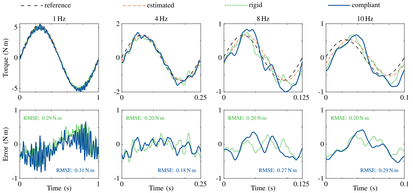
Fig. 6. Reference, estimated and both measured load cell torques of the compliant and rigid CMG at 1 Hz, 4 Hz, 8 Hz and 10 Hz, as well as the error between each load cell torque and the reference torque.
