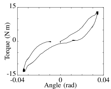
Fig. 9. Torque-deflection relation of the SPIDEX ®
